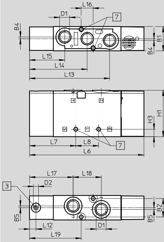
3 Port 14: pilot air 7 For mounting screw M4
